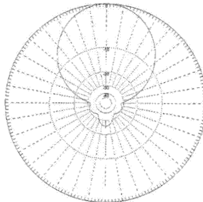
Figure 15.1: 3-Element Yagi
