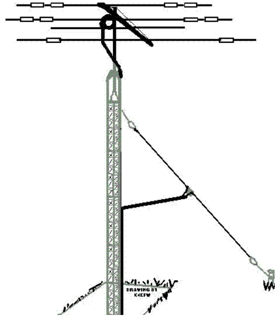
Figure 12.1: Half-Sloper Antenna
