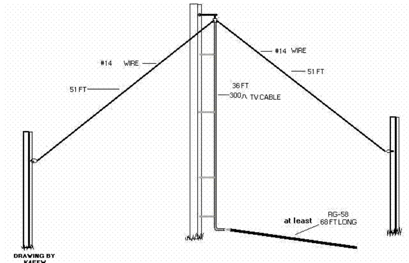
Figure 10.13: G5RV Dipole
